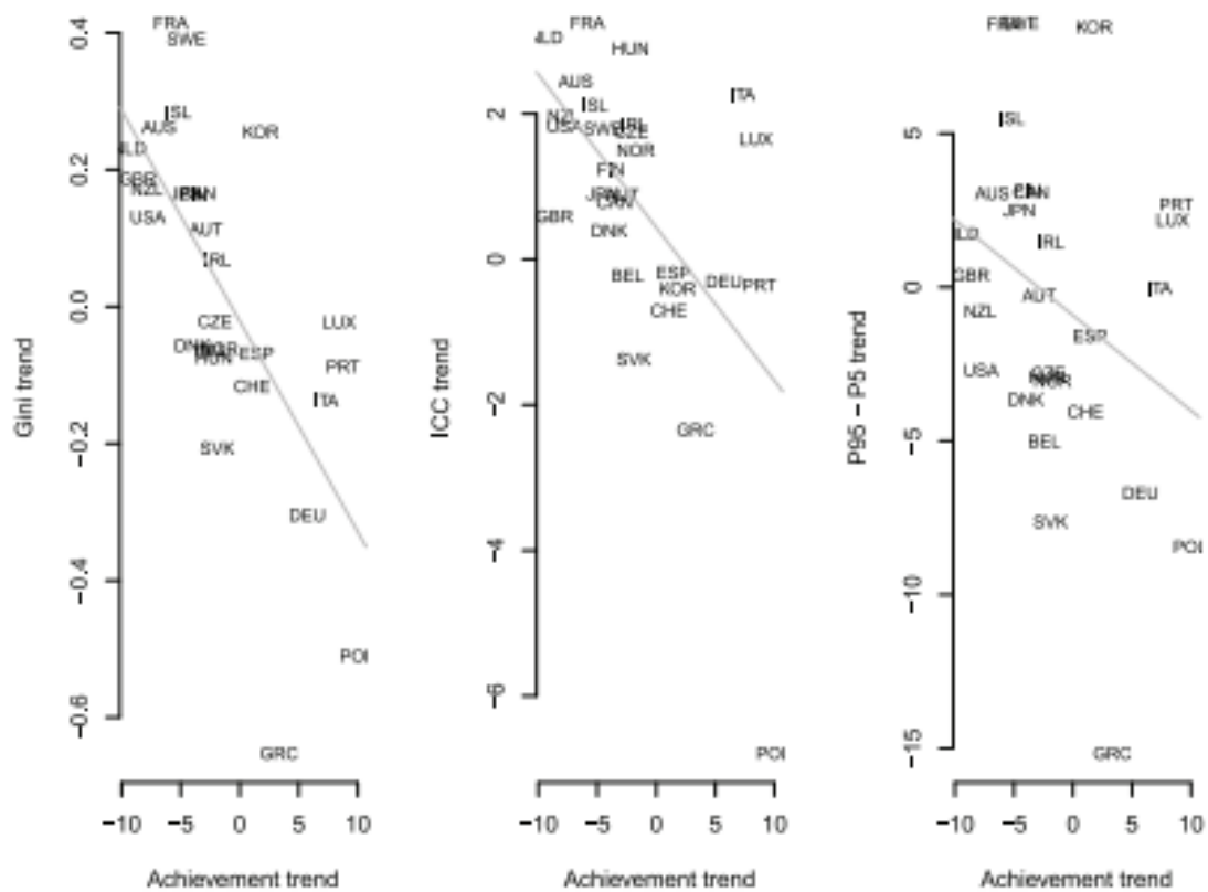
Figure 1. Math trends.
